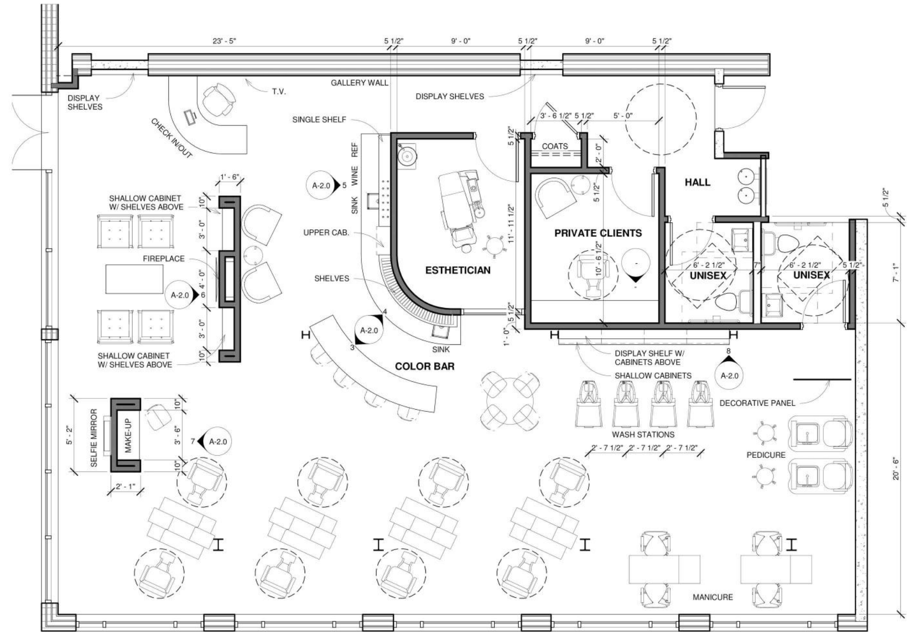
2 FIRST FLOOR 1/4" = 1'-0"
