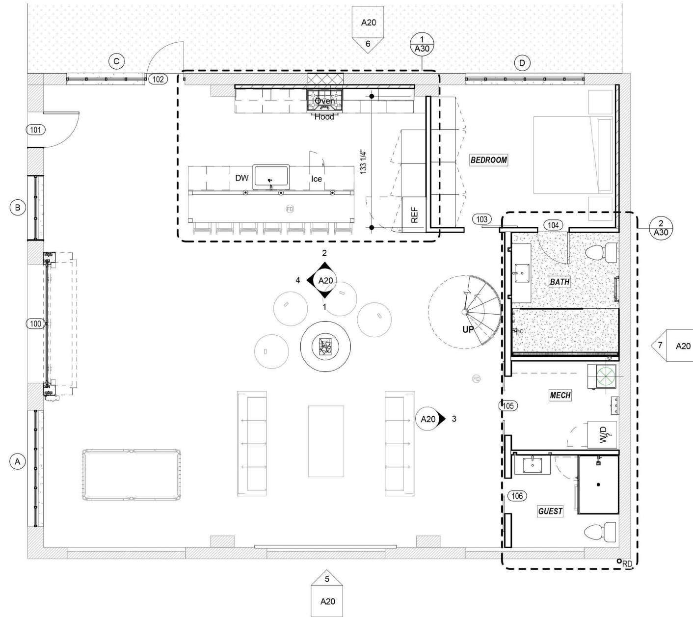
1 FLOOR PLAN 3/16" = 1'-0" 0' 1' 3' 6'
